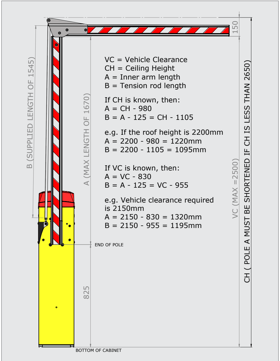
FIGURE 2. RECOMMENDED MINIMUM CLEARANCE
